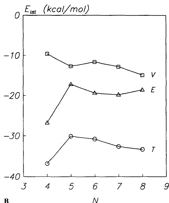
Fig. 4. (A) Buried surface areas for N=4, \dots, 8 helix bundles. The change in solvent accessible surface area per monomer upon helix bundle formation ( \Delta A ) is shown as a function of N . Changes in surface area for polar (P), non-polar (N) and the total for all atoms (T) are shown. (B) Monomer-monomer interaction energies ( E_{\text{int}} ) for the same helix bundles. The van der Waals (V) and electrostatic (E) components of the total interaction energy (T) per monomer-monomer interface are shown
